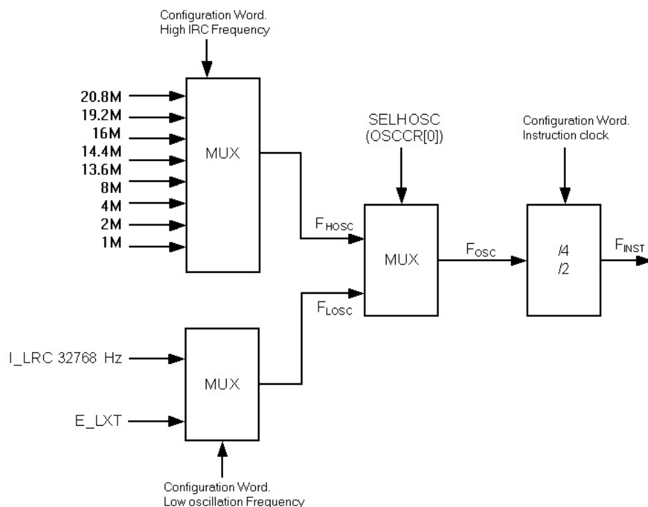
Figure 34 Oscillation Configuration of NY8B062A
