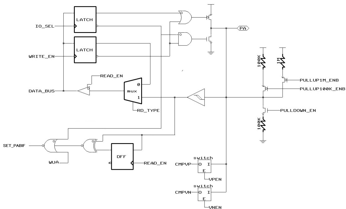
Figure 5 Block Diagram of PA2&PA0
