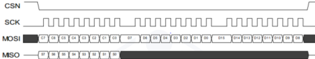
Figure 8.14 wire SPI read operation
