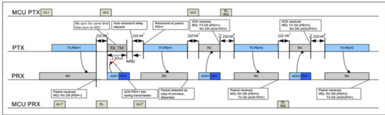
Figure 7.19 TX/RX cycles with ACK Payload and the according interrupts when the ACK packet fails
