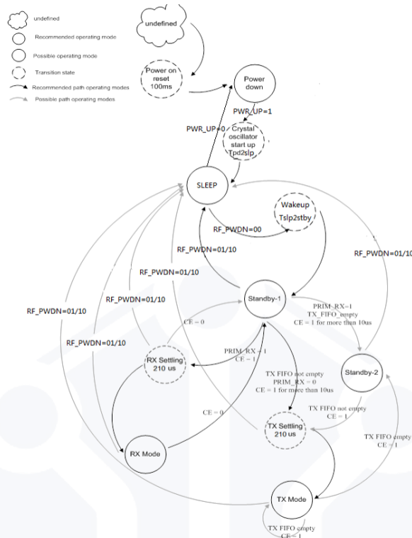
Figure 6.1 Radio control state diagram
