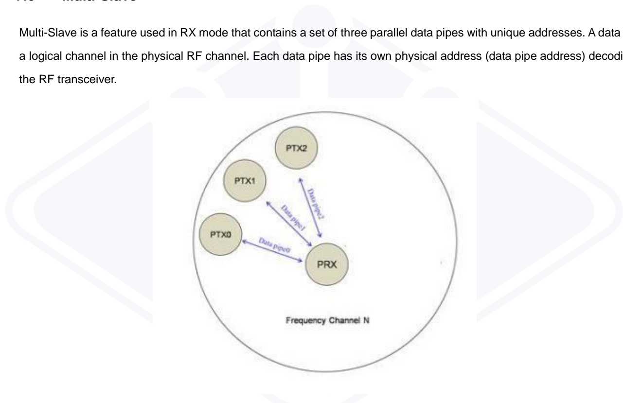
Figure7.8 PRX using Multi-Slave
