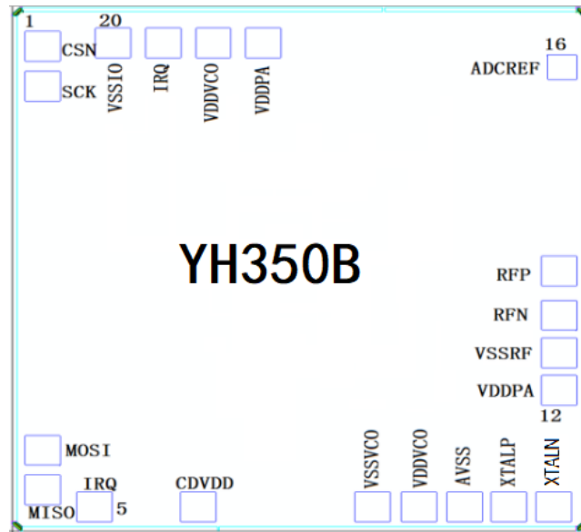
Figure2.1 YH350B pad assignment
