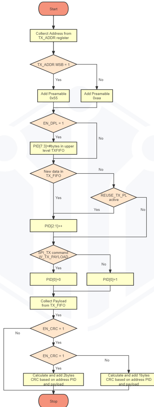
Figure 7.3 Automatic packet assembly
