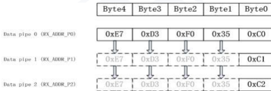
Figure 7.9 Addressing data pipes 0-2
