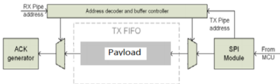
Figure 7.5 TX FIFO (PRX) with pending payloads
