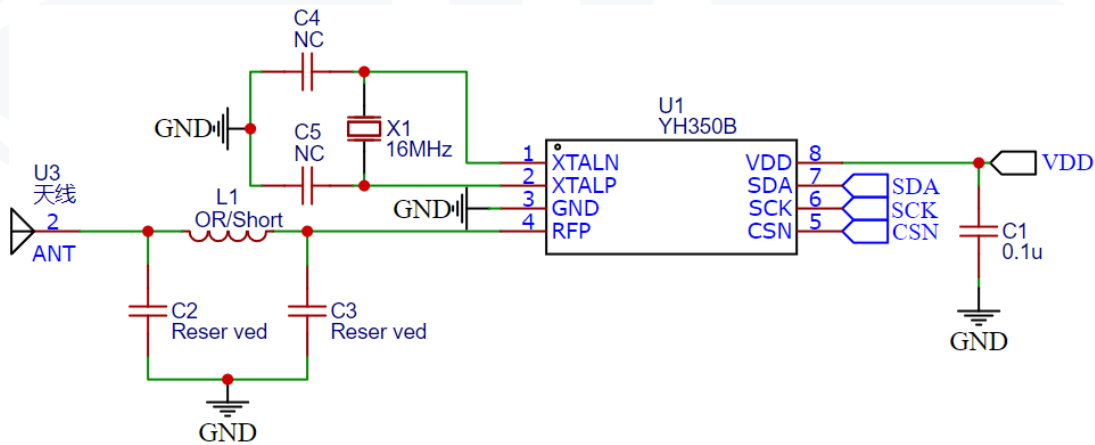
Figure2.3 YH350B SOP8 reference design
