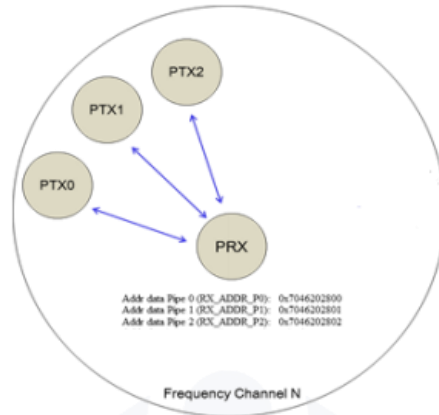
Figure 7.10 Example of data pipe addressing in Multi-Slave
